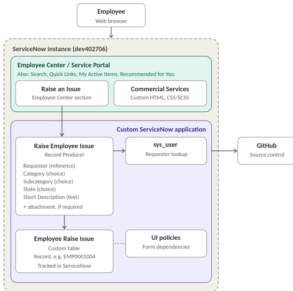
Figure 1: Solution architecture and data flow of the Employee Raise Issue Management System using ServiceNow
